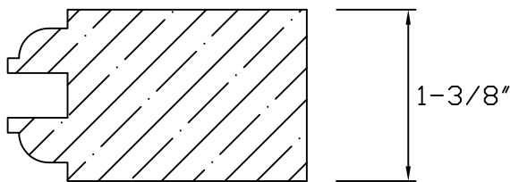
1 3/8" TDL #2 PROFILE
