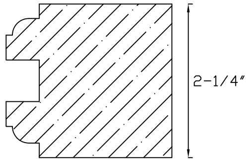
2 1/4" TDL #2 PROFILE
